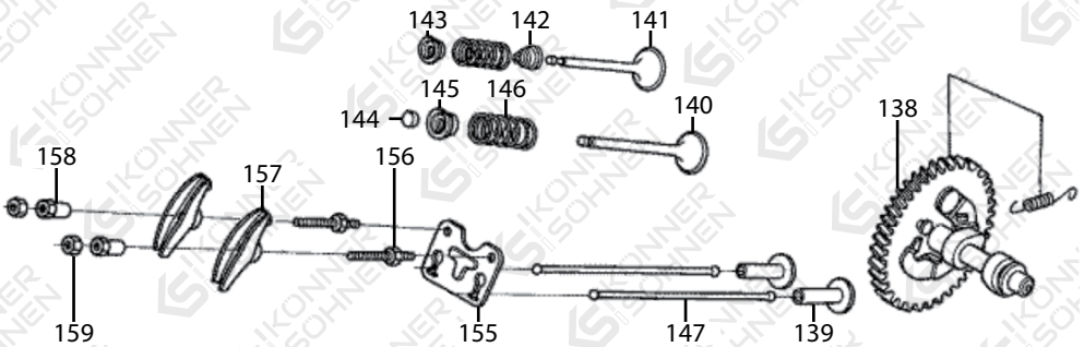
Pic. 1.2. Camshaft ASSY
