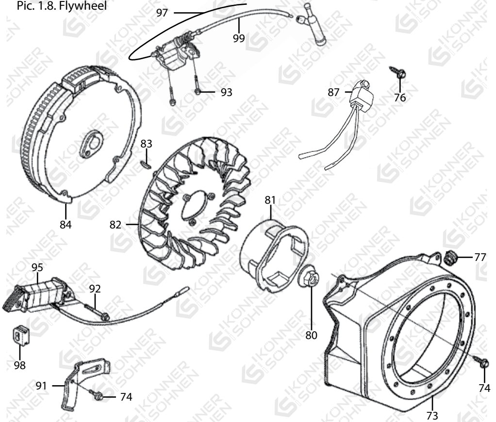
Pic. 1.8. Flywheel
